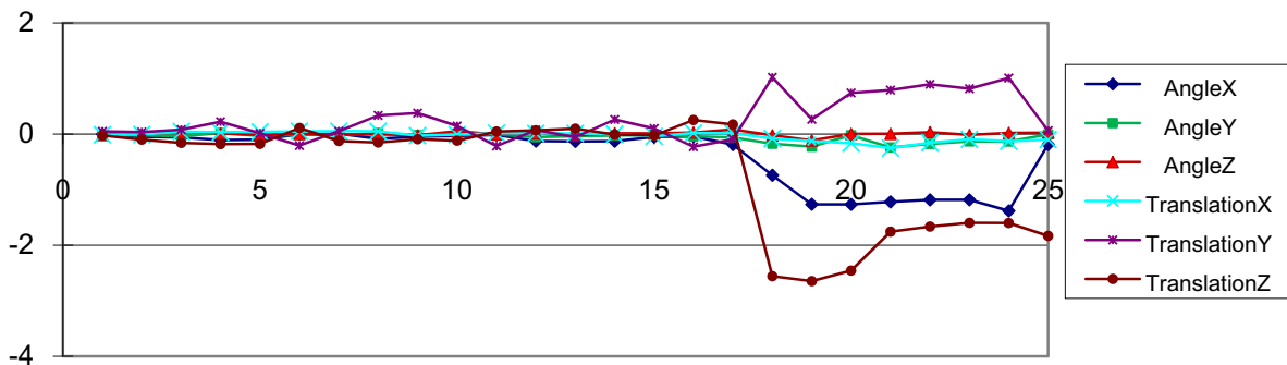
Figure 4. Motion parameters (in vertical) vs. gradient number (in horizontal) plot for gradient-wise checking shows large motion occurred after gradient-17. This kind of artifacts can be corrected by registering those gradient volumes to the baseline (usually the first volume if no baseline acquired in a multiple b-valued acquisition).
