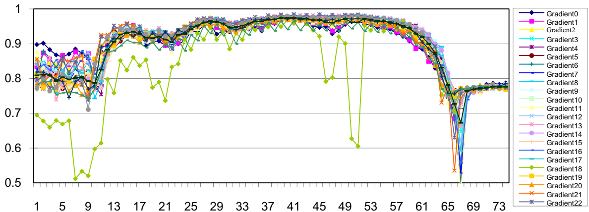
Figure 2. Correlation (in vertical) vs. slice number (in horizontal) plot for slice-wise checking shows that gradient-18 is abnormal at several slice locations indicating intensity artifacts in these slices.
