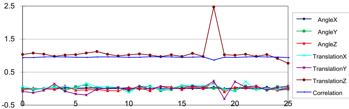
Figure 3. Motion parameters (in vertical) vs. gradient number (in horizontal) plot for interlace-wise checking shows a large translation in Z in gradient-18. Correlation (in vertical) vs. gradient number (in horizontal) plot also shows a drop for gradient-18. This implies that those slice intensity artifacts are very likely originating from motions between the interleaved acquisitions.
