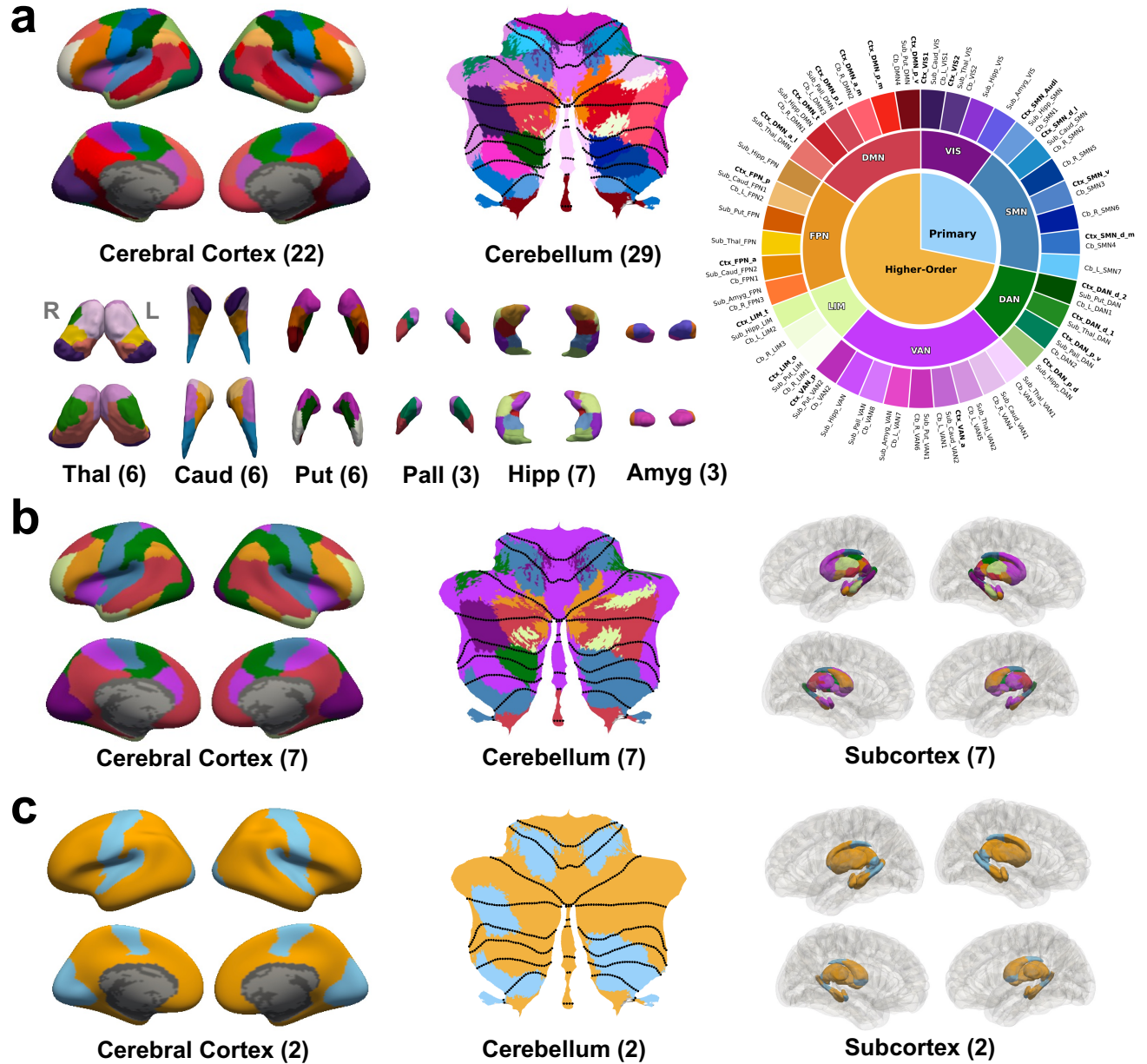
Figure 1. Overview of the UNC Early-Life Whole-Brain Functional (ELF) Parcellation.
